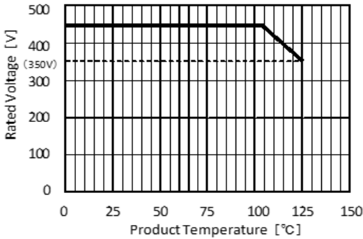
Fig:Derating
