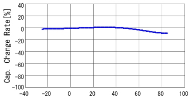
Temperature Characteristics
