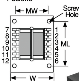
Mounting Style “B” 4 Screws
