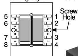
Schematic 1
