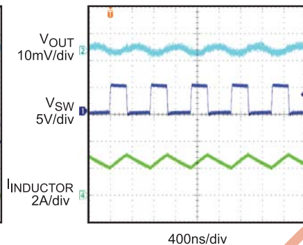
Switching Waveform
