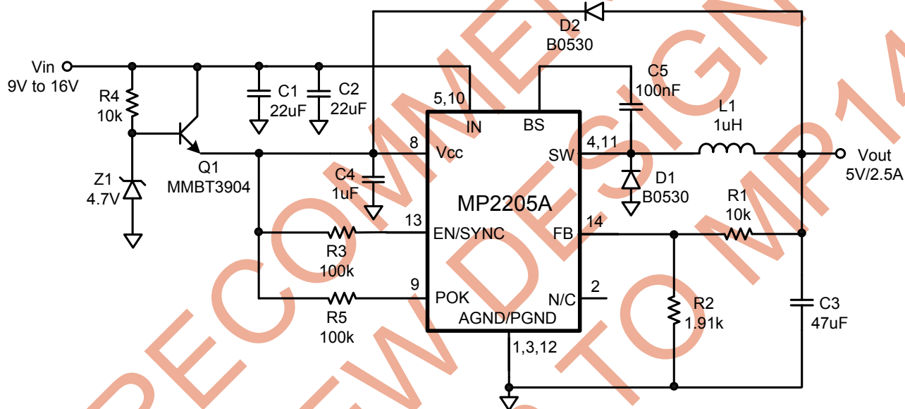
Figure 4—MP2205A with a Vcc Generation Circuit
