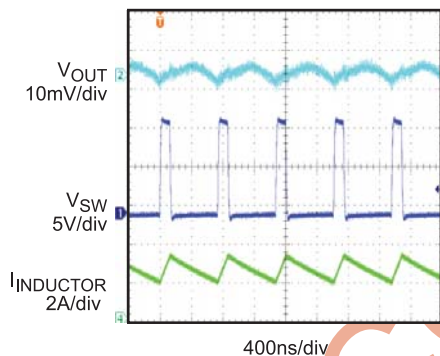
Switching Waveform
