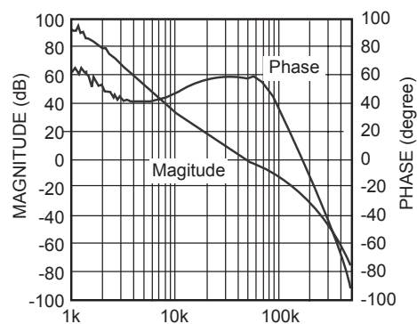
Close Loop Bode Plot
