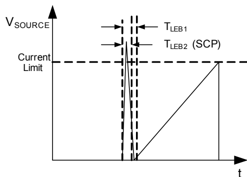
Figure 10: Leading-Edge Blanking
