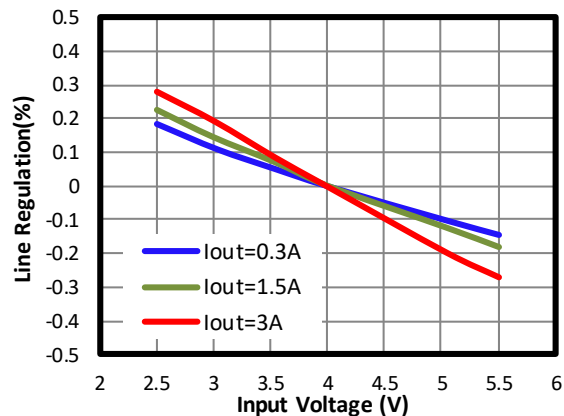
Line Regulation
