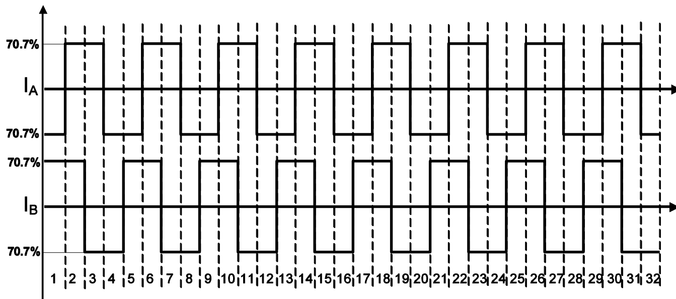
Figure 6a: Full-Step (4 Step Sequences)
