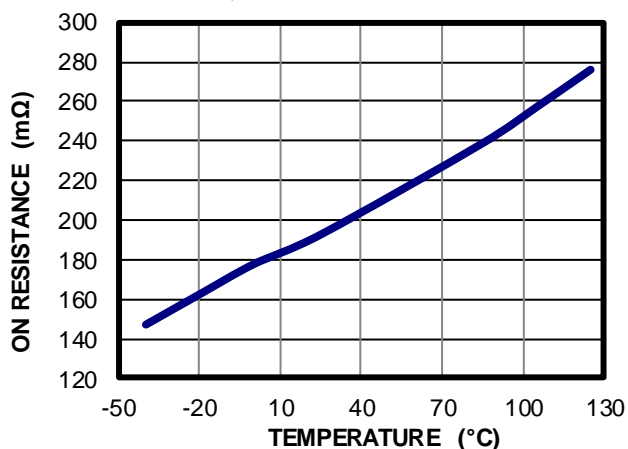
Bridge A LS On Resistance vs. Temperature
