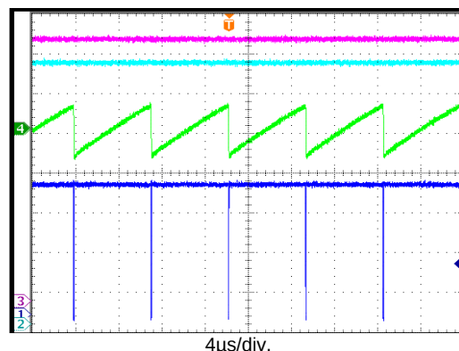
Dropout Operation
