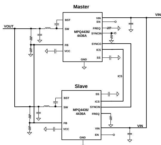
Figure 8: Dual-Phase Configuration
