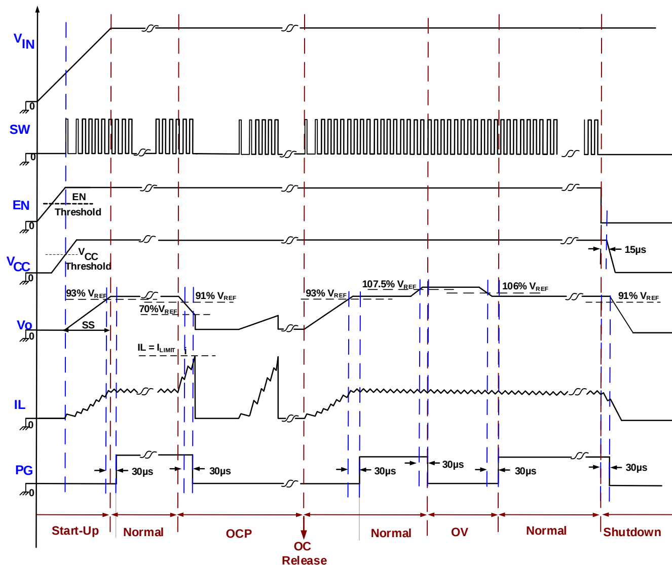
Figure 3: Timing Sequence
