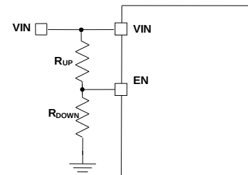
Figure 11: Adjustable UVLO Using EN Divider
