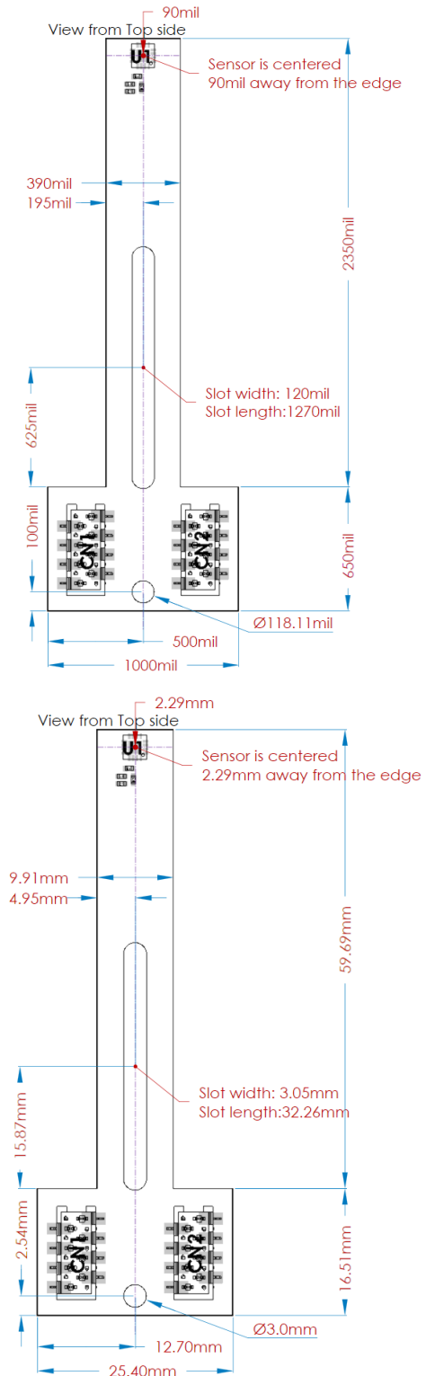
Figure 27: LT Type 3 Mechanical Drawing, mil = 0.001" = 0.0254mm
