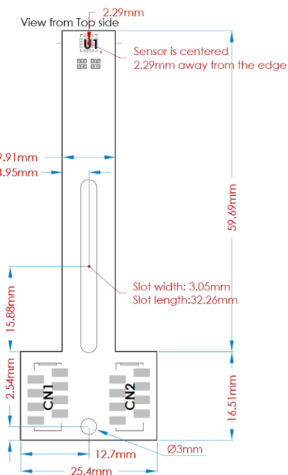
Figure 9: LT Type 1 Mechanical Drawing, mil = 0.001" = 0.0254mm
