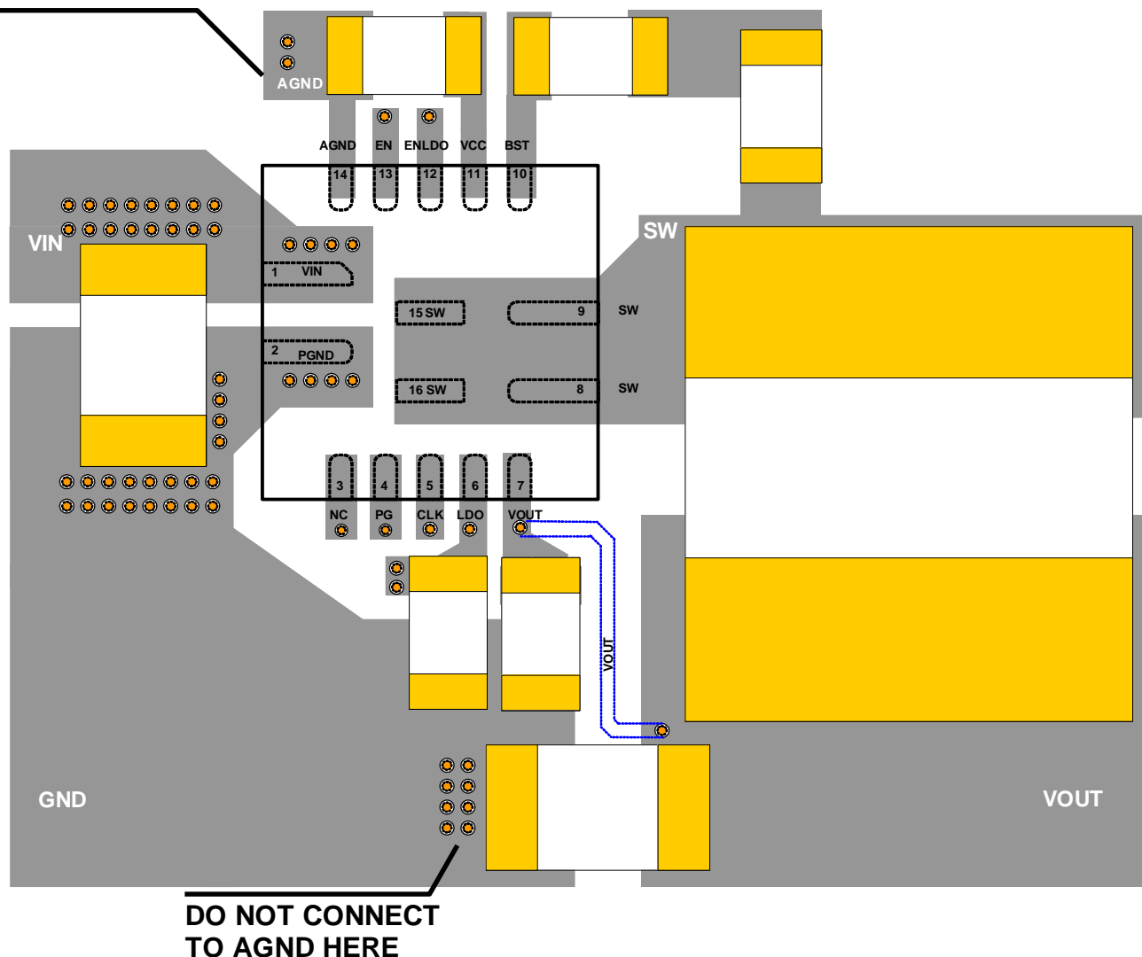
Figure 9—Recommend Layout
