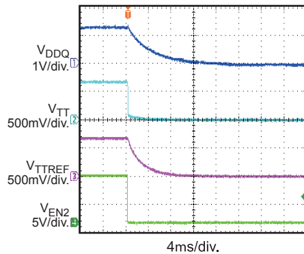
V_{TT} & V_{TTREF} Shutdown through EN2
