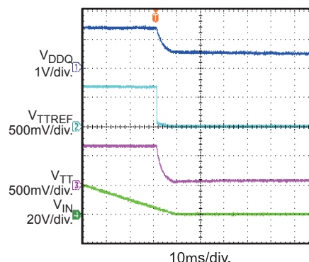
V TT &V TTREF Shutdown through V IN
