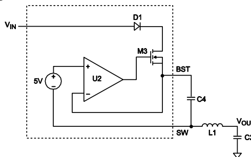
Figure 2—Internal Bootstrap Charging Circuit
