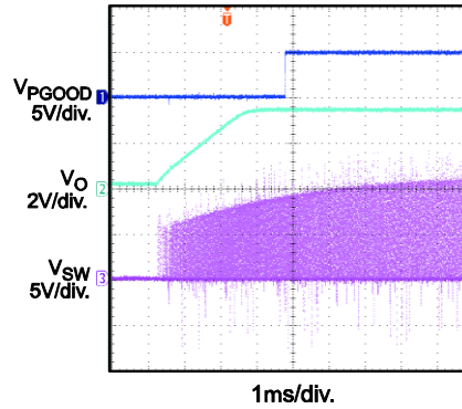
Power Startup – Full Load
