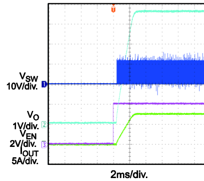
EN Startup with I_O = 7A
