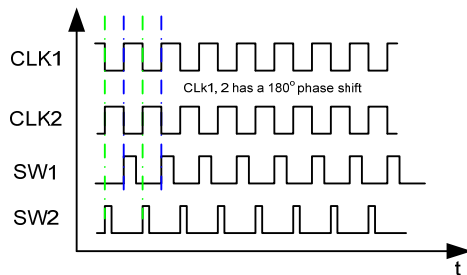
Figure 2: 180° Out-of-Phase Operation
