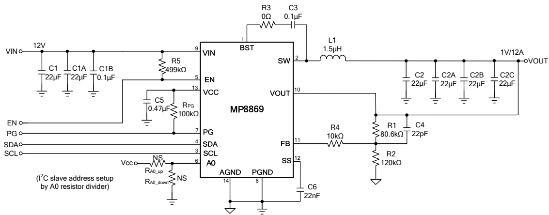
Figure 14: V_{IN} = 12V , V_{OUT} = 1V , I_{OUT} = 12A
