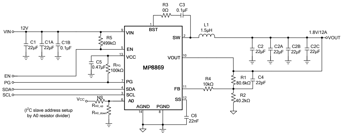
Figure 17: V_{IN} = 12V , V_{OUT} = 1.8V , I_{OUT} = 12A
