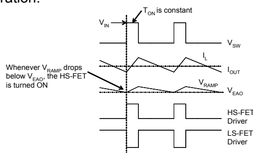
Figure 3: Forced PWM Operation
