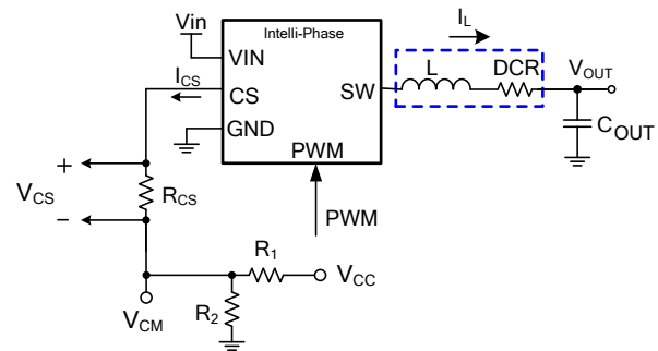
Fig.3 Use VCC to generate VCM voltage for CS signal
