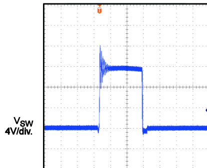
Switching Waveform
