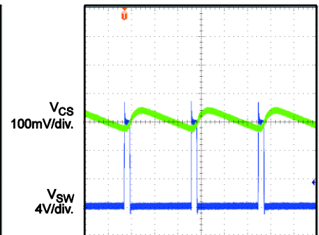
CS Output Waveform
