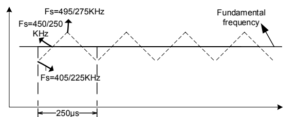
Figure 5, Frequency Spread Spectrum
