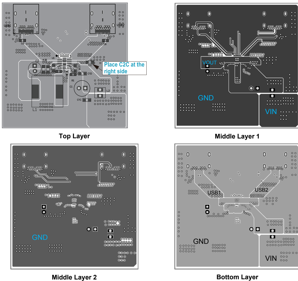
Figure 12: Recommended Layout
