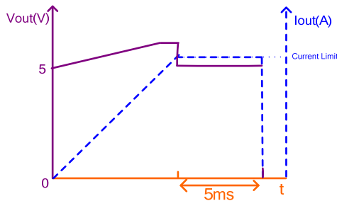
Figure 7: Over-Current Limit
