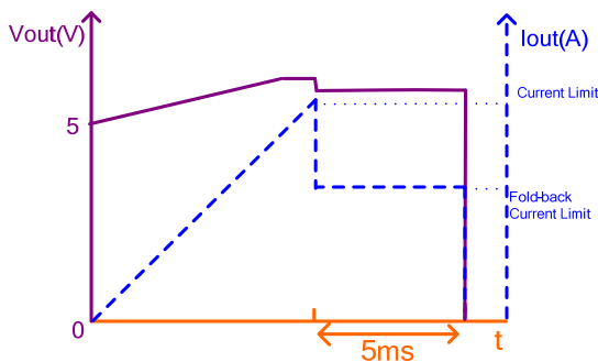
Figure 4: Over-Current Limit
