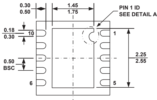
TQFN10 (3mm x 3mm)
