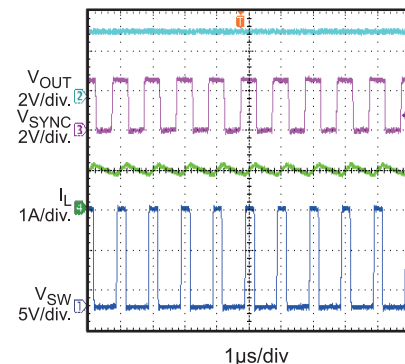
SYNC Operation (In-Phase)
