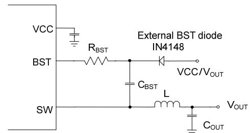
Figure 7: External Bootstrap Diode and Resistor
