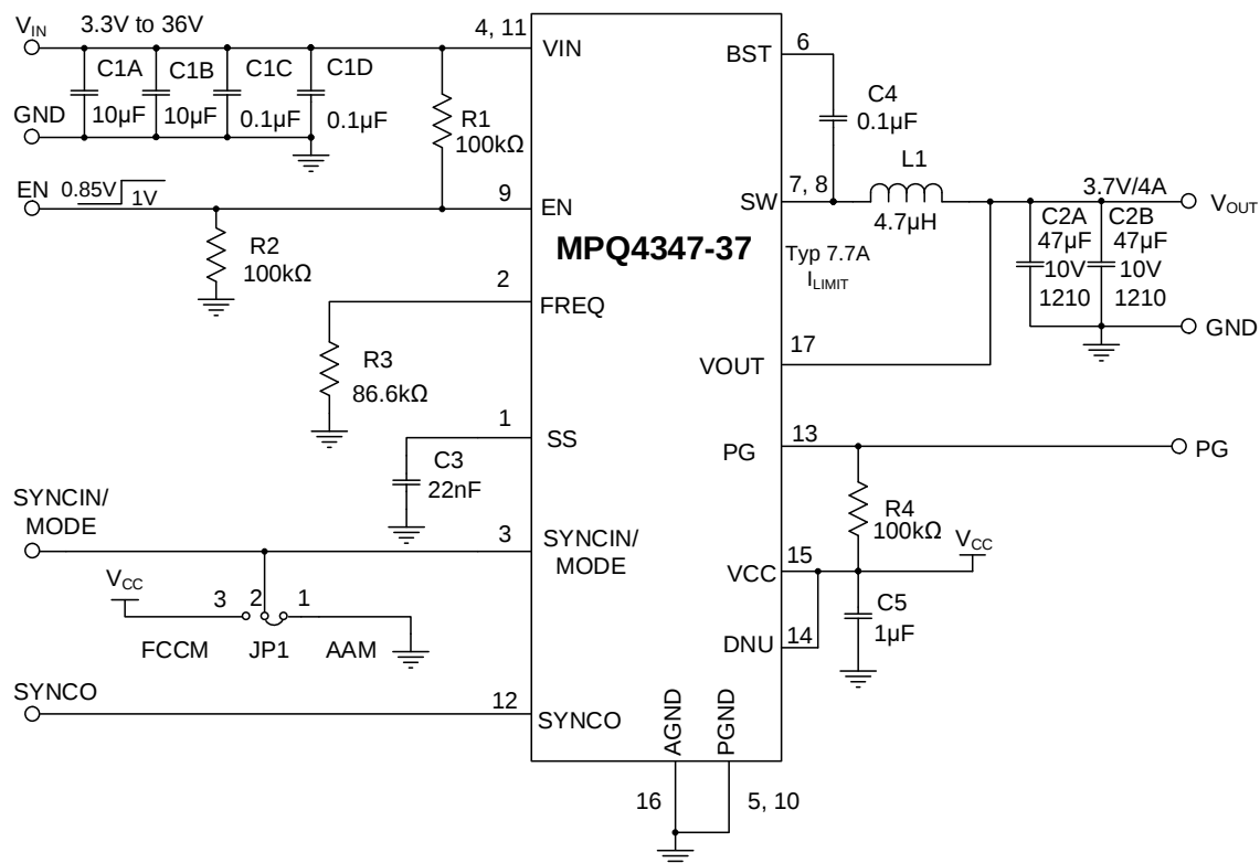
Figure 12: Typical Application Circuit ( V_{OUT} = 3.7V , f_{SW} = 410kHz )
