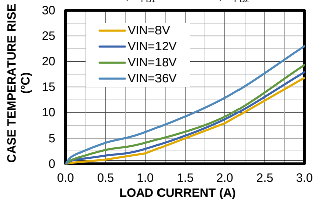
Case Temperature Rise vs. Load Current
