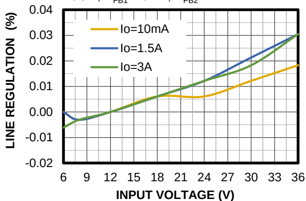
Line Regulation vs. Input Voltage
