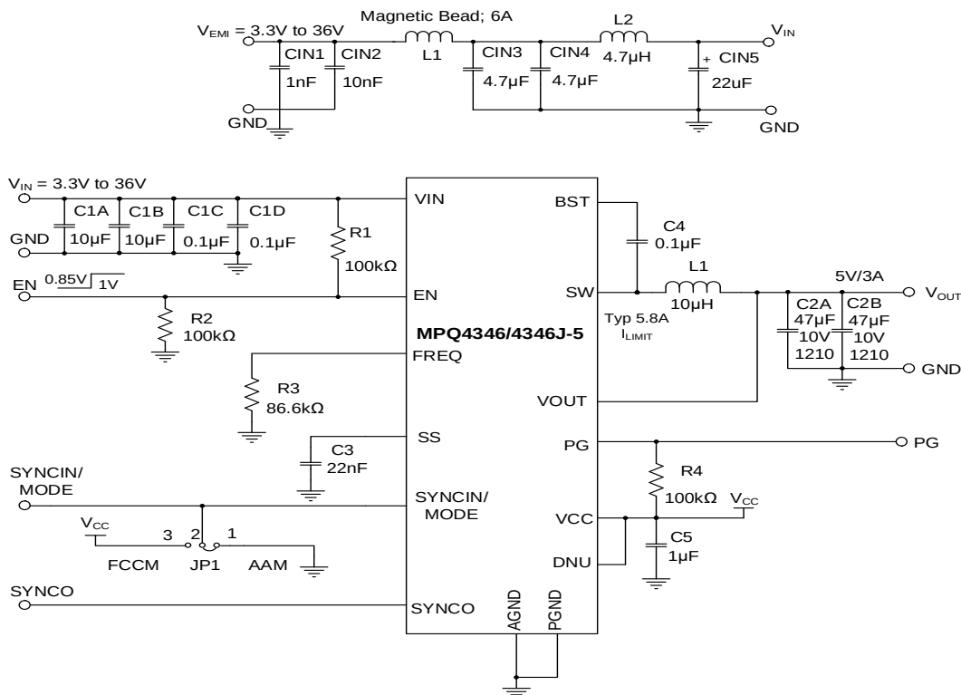
Figure 14: Typical Application Circuit ( V_{OUT} = 5V , f_{sw} = 410kHz with EMI Filter)
