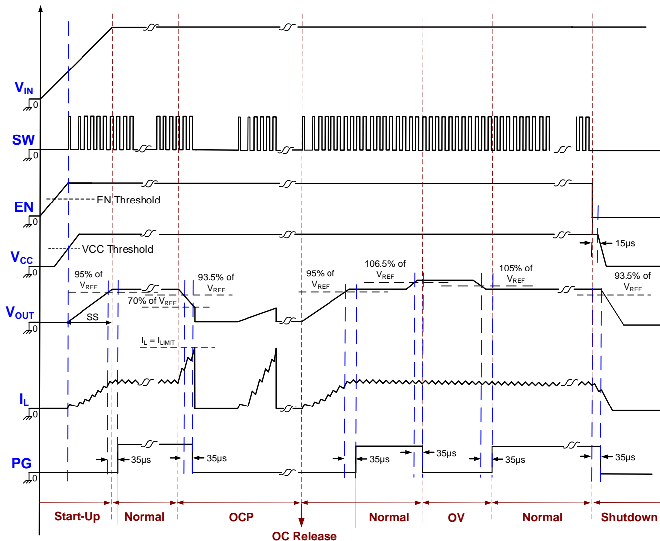
Figure 2: Timing Diagram
