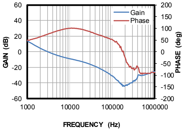
Bode Plot
