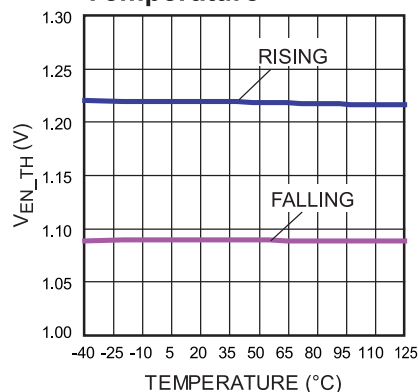
EN/SYNC Threshold vs. Temperature
