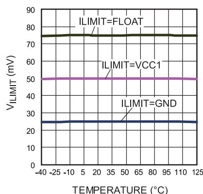
Current Limit Sense Voltage vs. Temperature
