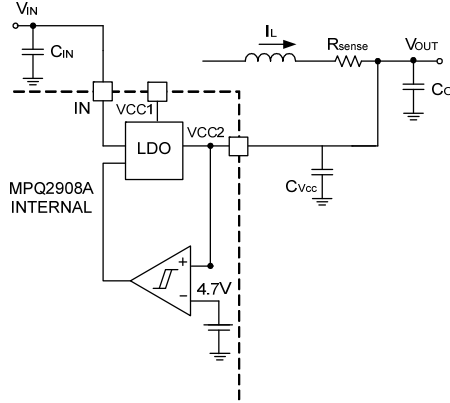
Figure 7: Configuration of VCC2 Connecting to V_{OUT}
