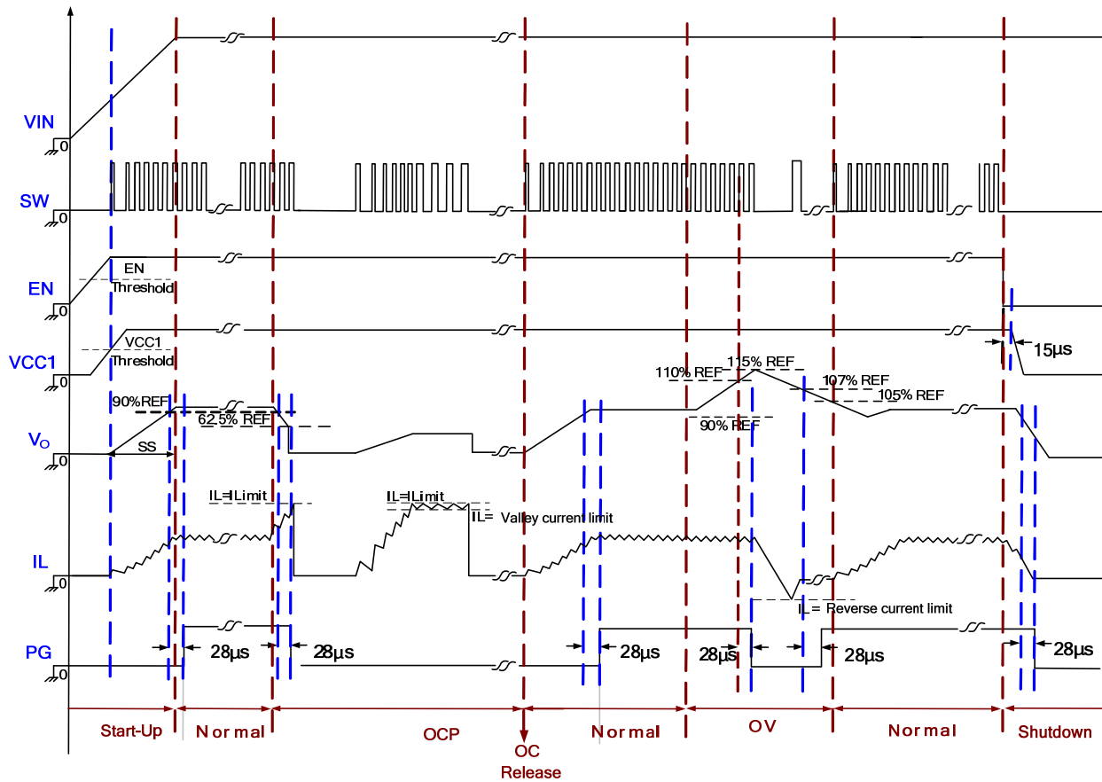
Figure 2: Time Sequence
