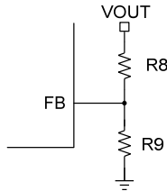
Figure 5: External Resistor Divider
