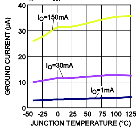
Ground Current vs. Junction Temperature V_{IN}=6V, V_{OUT}=5V
