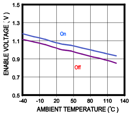
Enable Voltage vs. T_A
