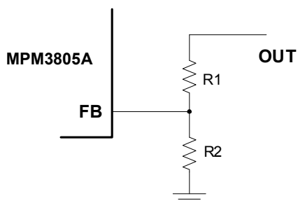
Figure 2: Feedback Network
