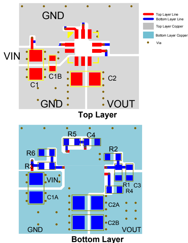
Figure 6: Recommended Layout
