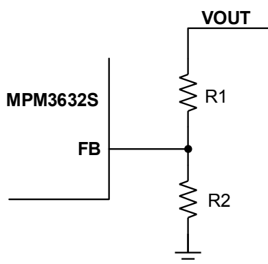
Figure 5: Feedback Network
