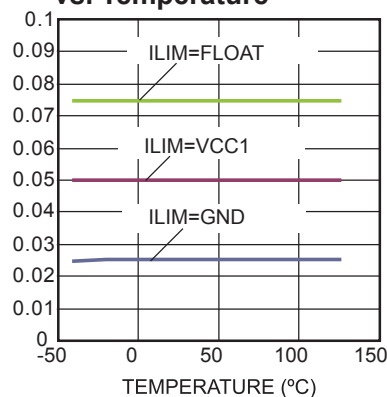
Internal Current Limit vs. Temperature
