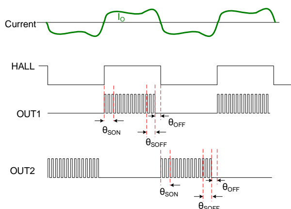
Figure 2: Timing Diagram
