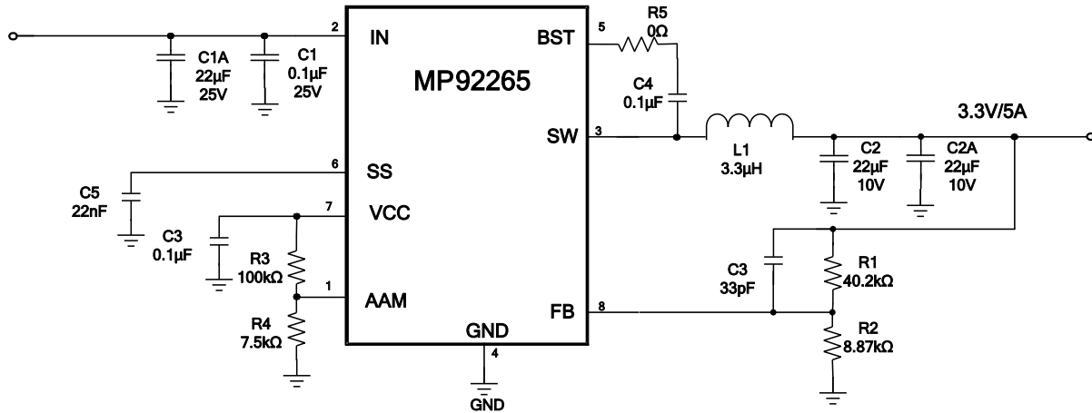
Figure 8: 12 V_{IN} , 3.3V/5A
