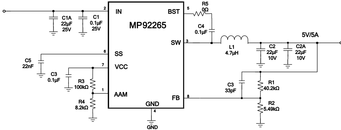
Figure 7: 12 V_{IN} , 5V/5A
