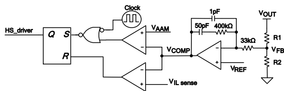
Figure 2: Simplified AAM Control Logic
