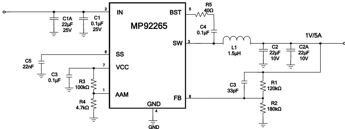
Figure 9: 12 V_{IN} , 1V/5A (9)
