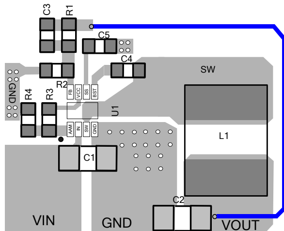
Figure 6: Recommended Layout
