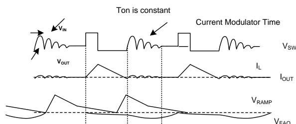
Figure 5: Light-Load Operation
