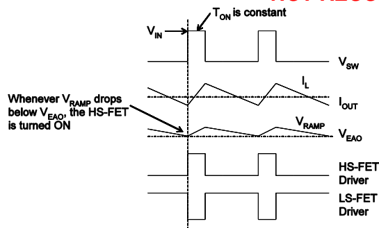
Figure 4: Forced PWM Operation
