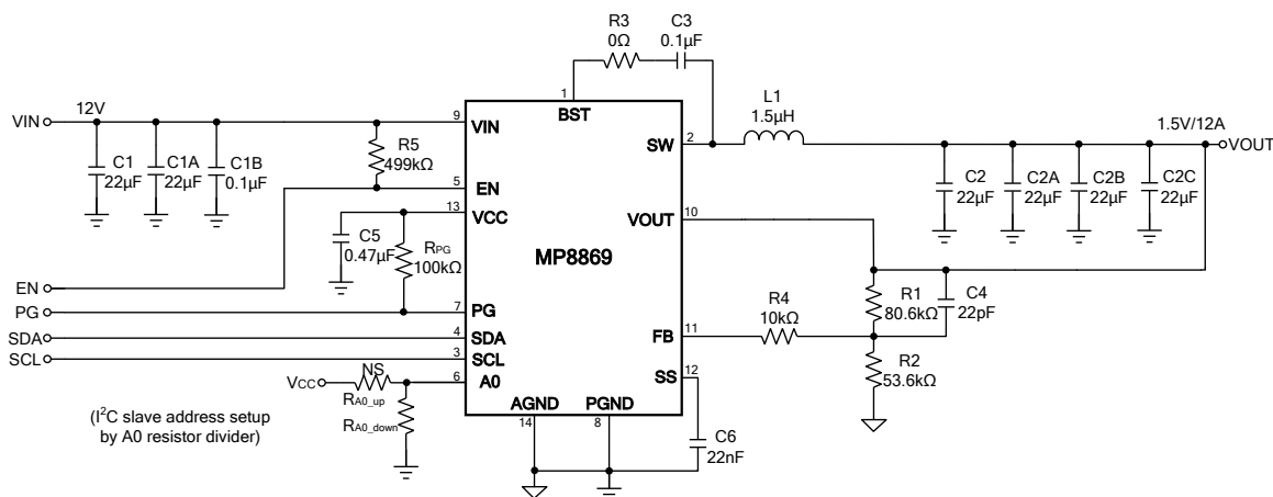
Figure 16: V_{IN} = 12V , V_{OUT} = 1.5V , I_{OUT} = 12A
