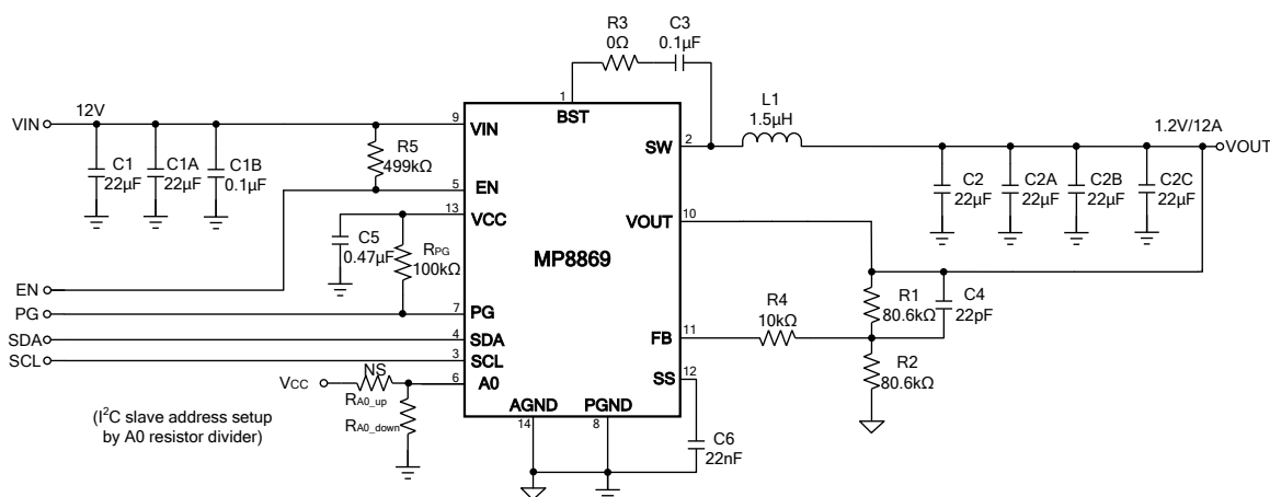
Figure 15: V_{IN} = 12V , V_{OUT} = 1.2V , I_{OUT} = 12A
