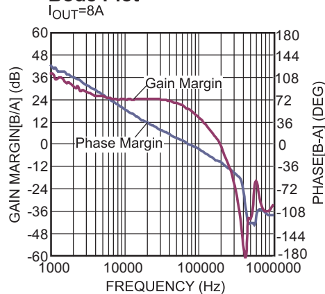
Bode Plot
