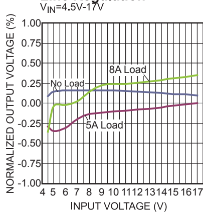
Line Regulation
