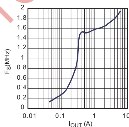
F_S vs. Load
