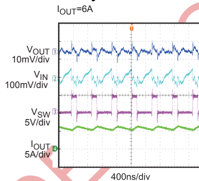
Steady State I_{OUT}=6A
