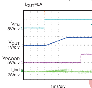
PGOOD, Startup Through EN I_{OUT}=0A
