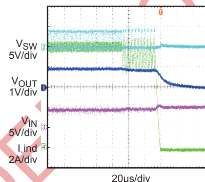
Over-current Protection
