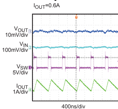
Steady State I_{OUT}=0.6A
