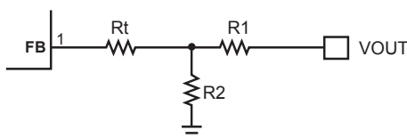
Figure 3— T-type Network
