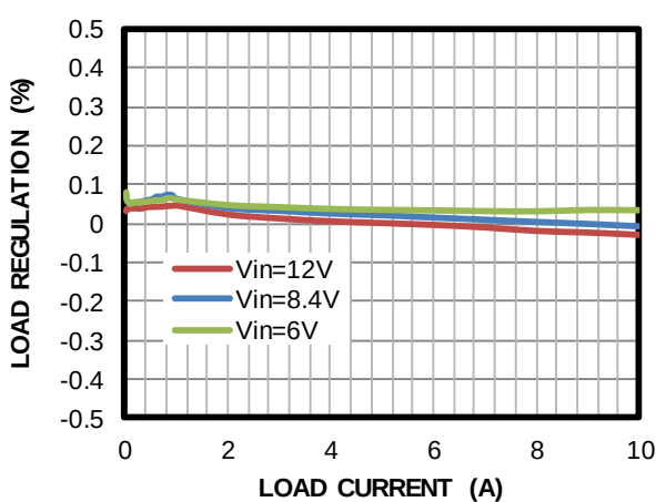
Load Regulation
