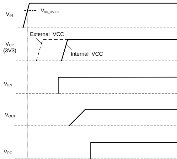
Figure 7: Start-Up Sequence
