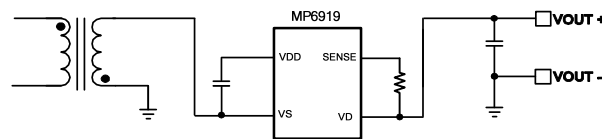
Figure 4: High-Side Rectification
