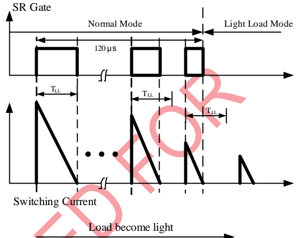
Figure 5—Enter Light Load Mode
