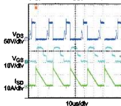
Operation in 90W Flyback Application
