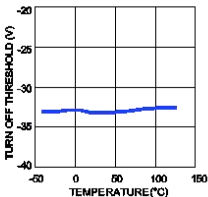
Turn-Off Threshold vs. Temperature
