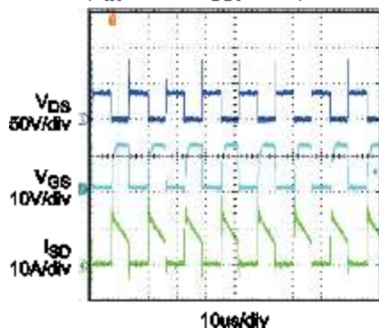
Operation In 90W Flyback Application
