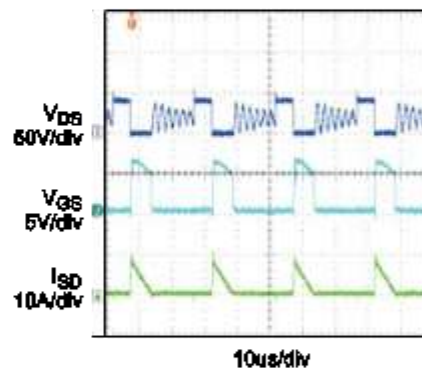
Operation in 90W Flyback Application (7)
