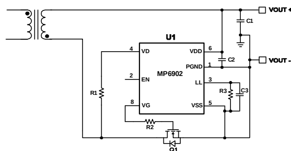
Figure 8— IC Supply derived directly from Output Voltage
