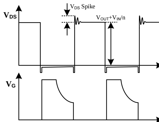
Figure 5—Drain-Source and Gate Driver voltage on SR MOFET
