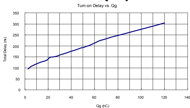
Figure 7—Total Turn-on Delay vs. Qg
