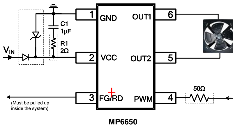
Figure 9: Typical Application Circuit for 12V VCC Input
