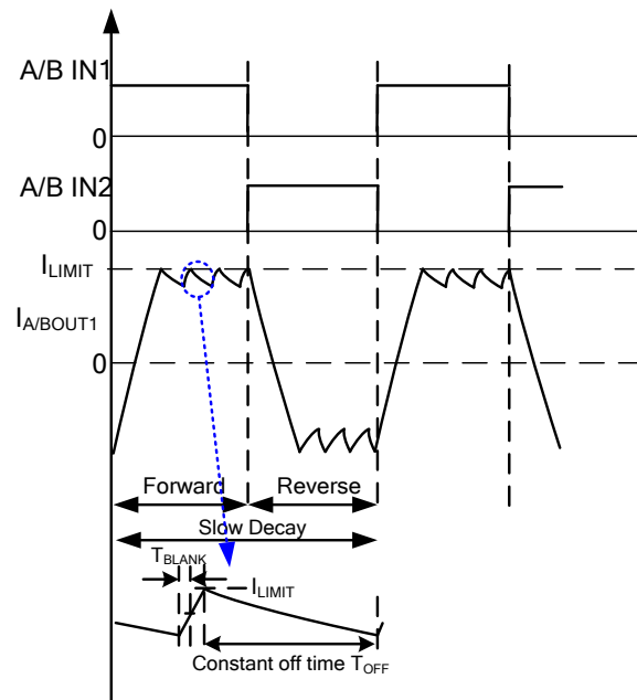
Figure 6: Internal PWM Current Control Waveform
