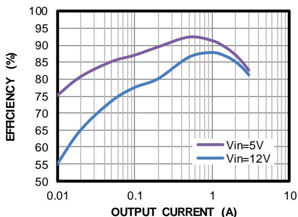
Efficiency, V OUT = 1.8V
