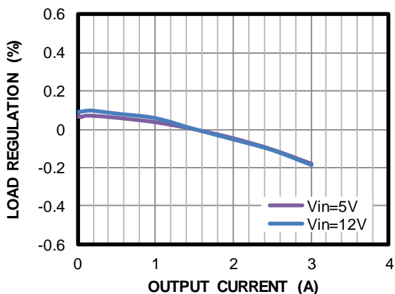
Load Regulation
