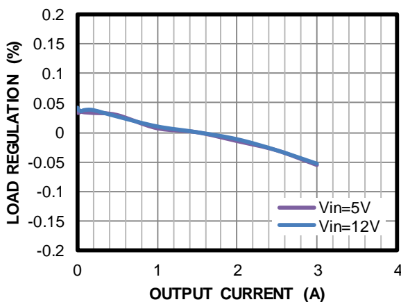
Load Regulation
