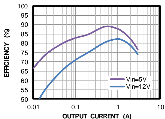
Efficiency, V OUT = 5V
