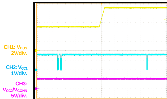
PDO Transition
