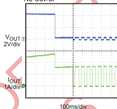
Current Limit (trip→hold→thermal shut down) →Auto Start Up
