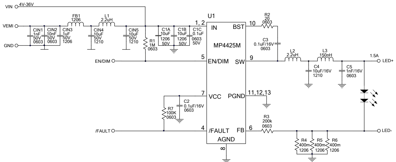
Figure 8: I_o=1.5A Application Circuit
