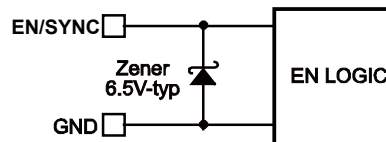
Figure 2: 6.5V-Type Zener Diode
